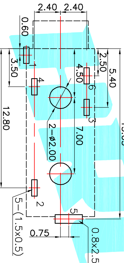
P.C.B LAYOUT(copper-sided view)
