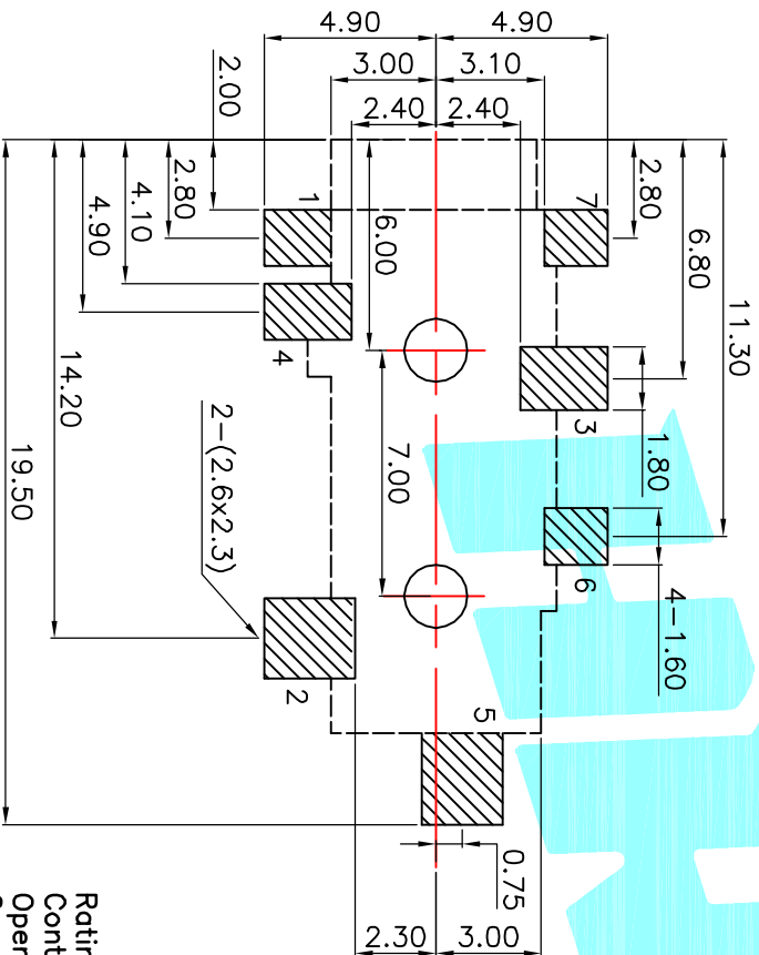
P.C.B Layout (copper-sided view)
