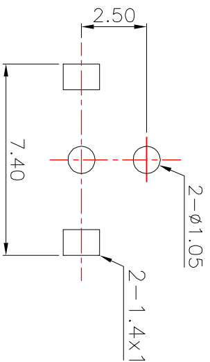
HOLE LAYOUT
