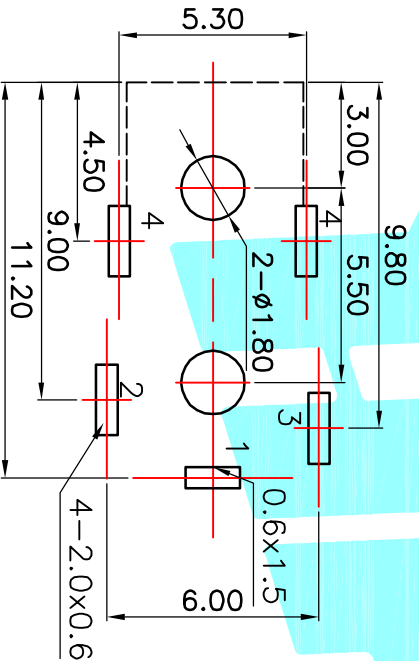
P.C.B LAYOUT(Copper-side view)
