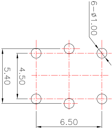
PCBLayout(Pattern Side)
